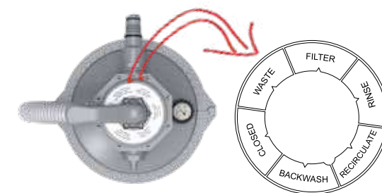
6-position valve
